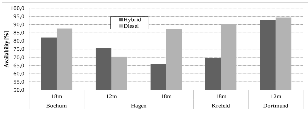
Figure 9: Availability, long term data
