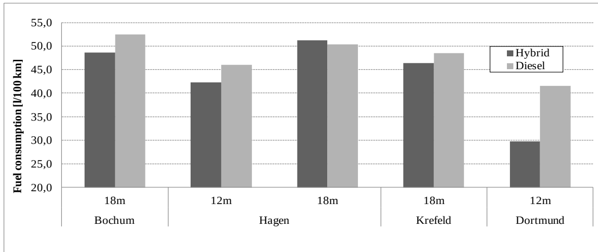
Figure 8: Fuel consumption, long term data
