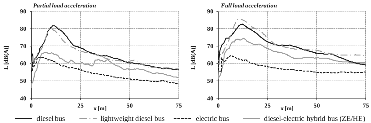
Figure 7: Measured exterior noise for bus departures with partial and full load acceleration
