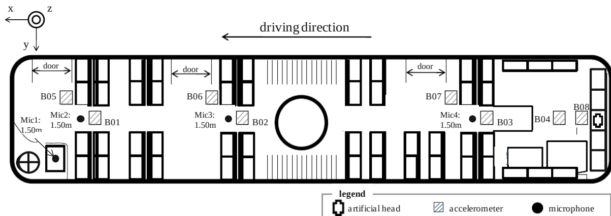
Figure 3: Measuring positions interior noise and vibrations
