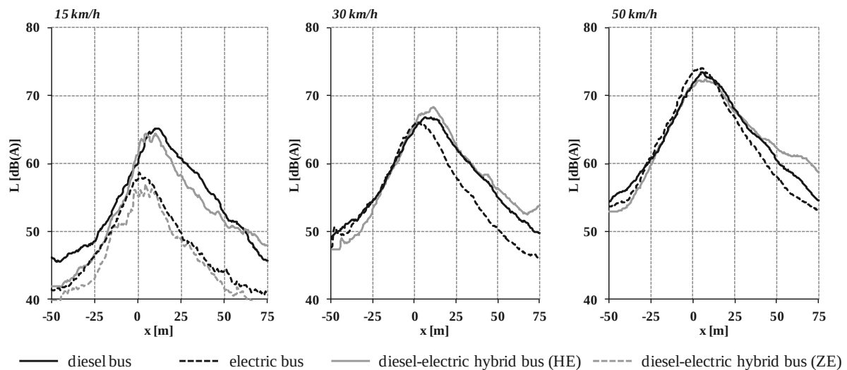
Figure 6: Measured exterior noise for pass-by tests with constant speeds
