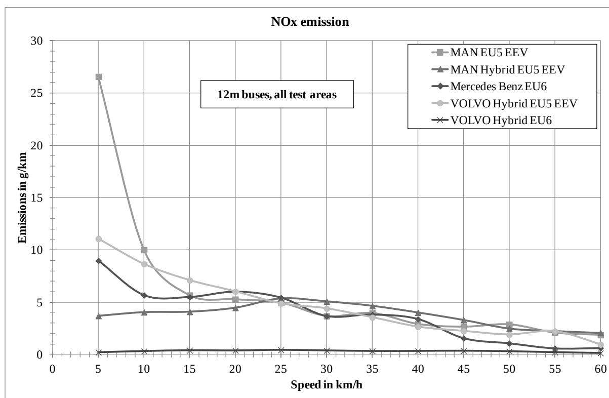
Figure 5: NO x Emissions as a function of vehicle speed, 12m buses, all test areas
