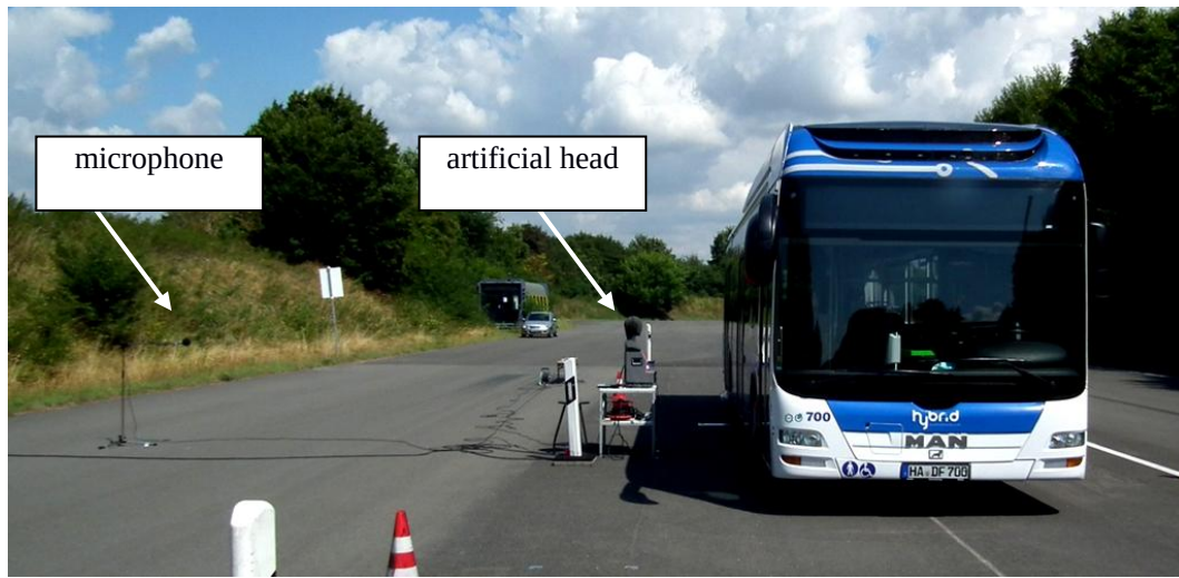
Figure 2: Measuring positions exterior noise
