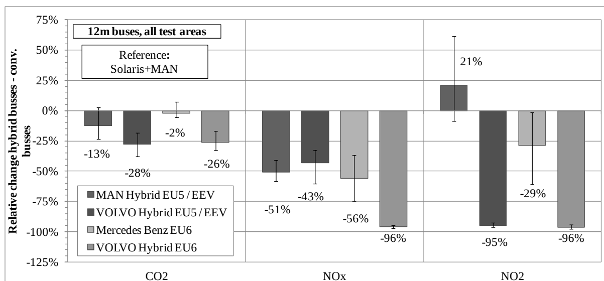
Figure 4: Emission measurement results for 12m buses, all test areas
