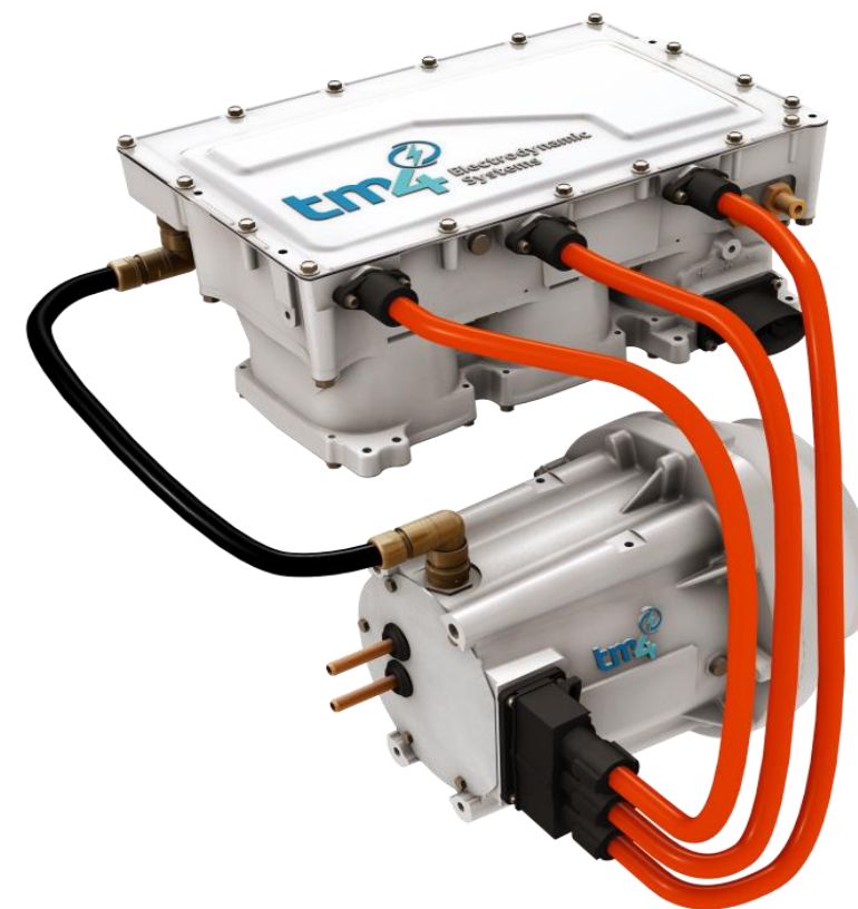
Inverter/Motor
