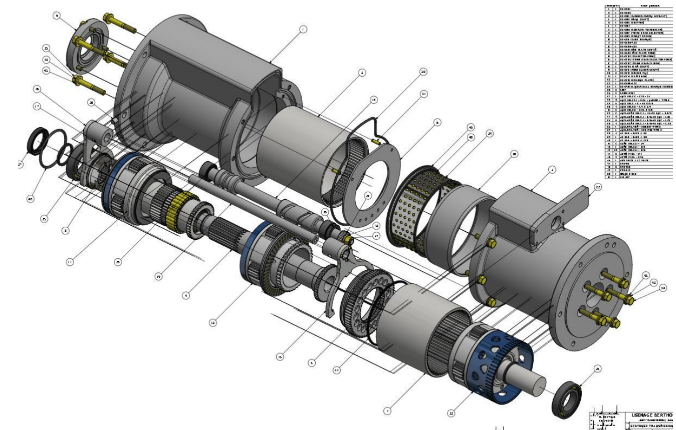
Transmission
